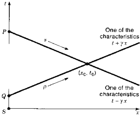
Figure 3. Characteristics in the dimensionless position-time plane.
