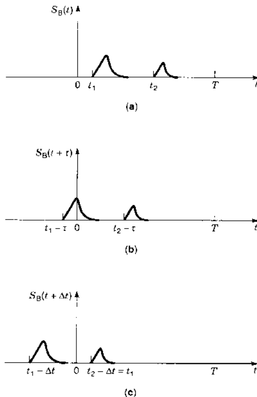
Figure 5. (a) Typical backward wave. (b) Shifted backward wave. (c) The product of S_B(t) and S_B(t + \tau) is maximum when \tau = \Delta t and second and first reflections are aligned.
