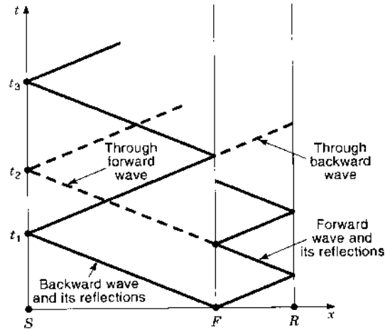
Figure 4. Lattice diagram.
