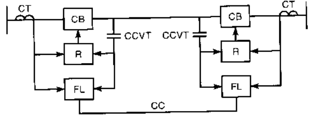
Figure 1. Fault-location equipment connection. CB is the circuit breaker, R the relay, FL the fault location, CT the current transformer, CCVT the capacitor coupling voltage transformer, and CC the communication channel (not always required).
